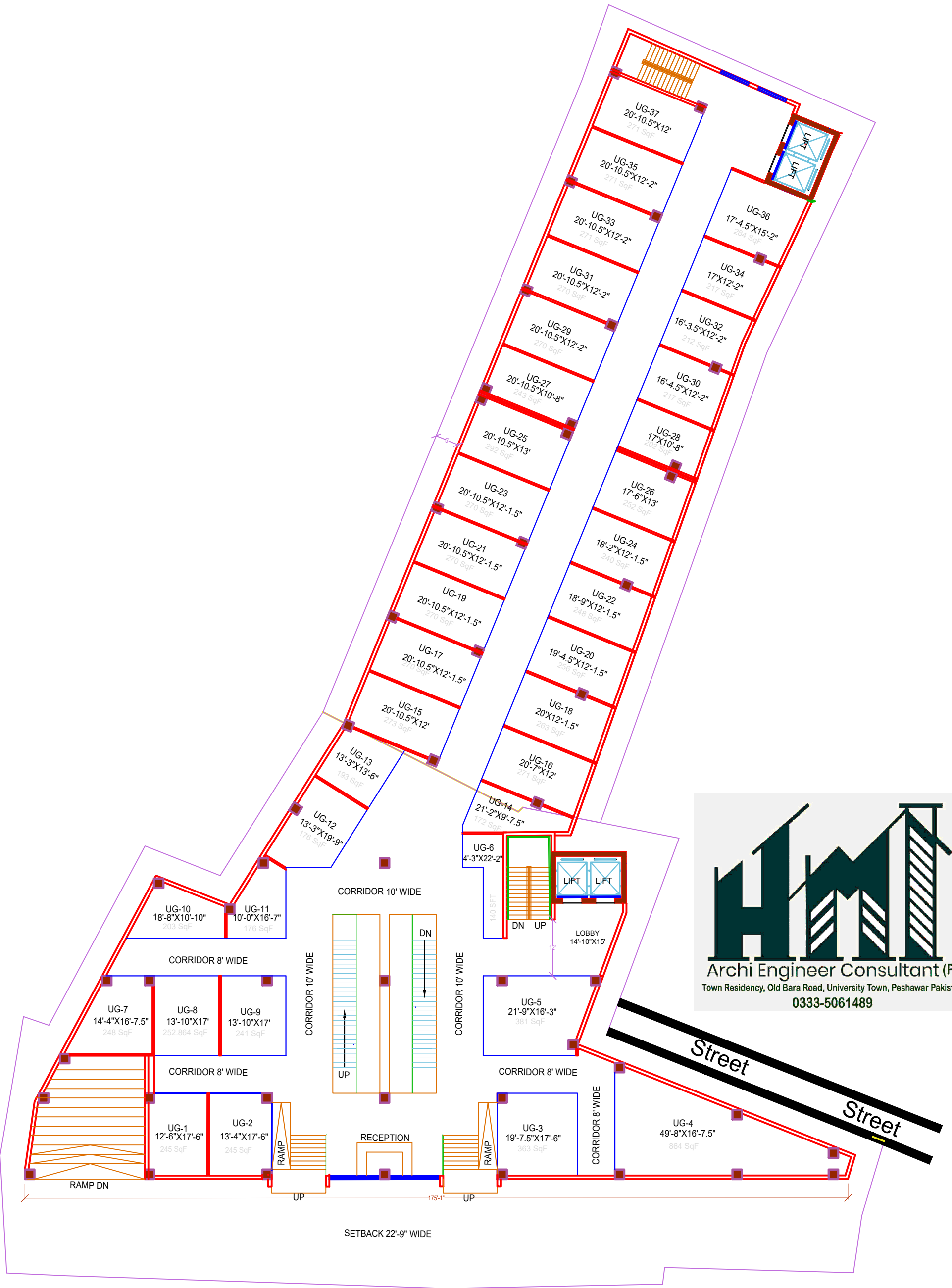
GROUND FLOOR PLAN SHOPS
