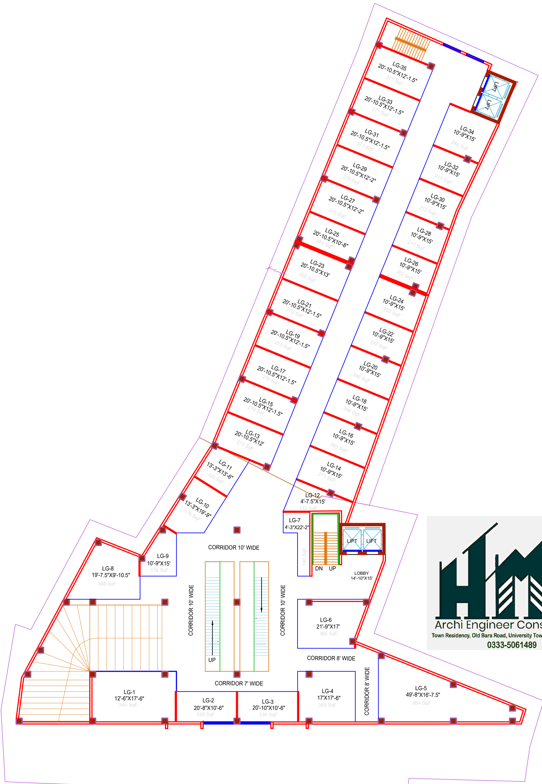
LOWER GROUND FLOOR PLAN SHOPS
