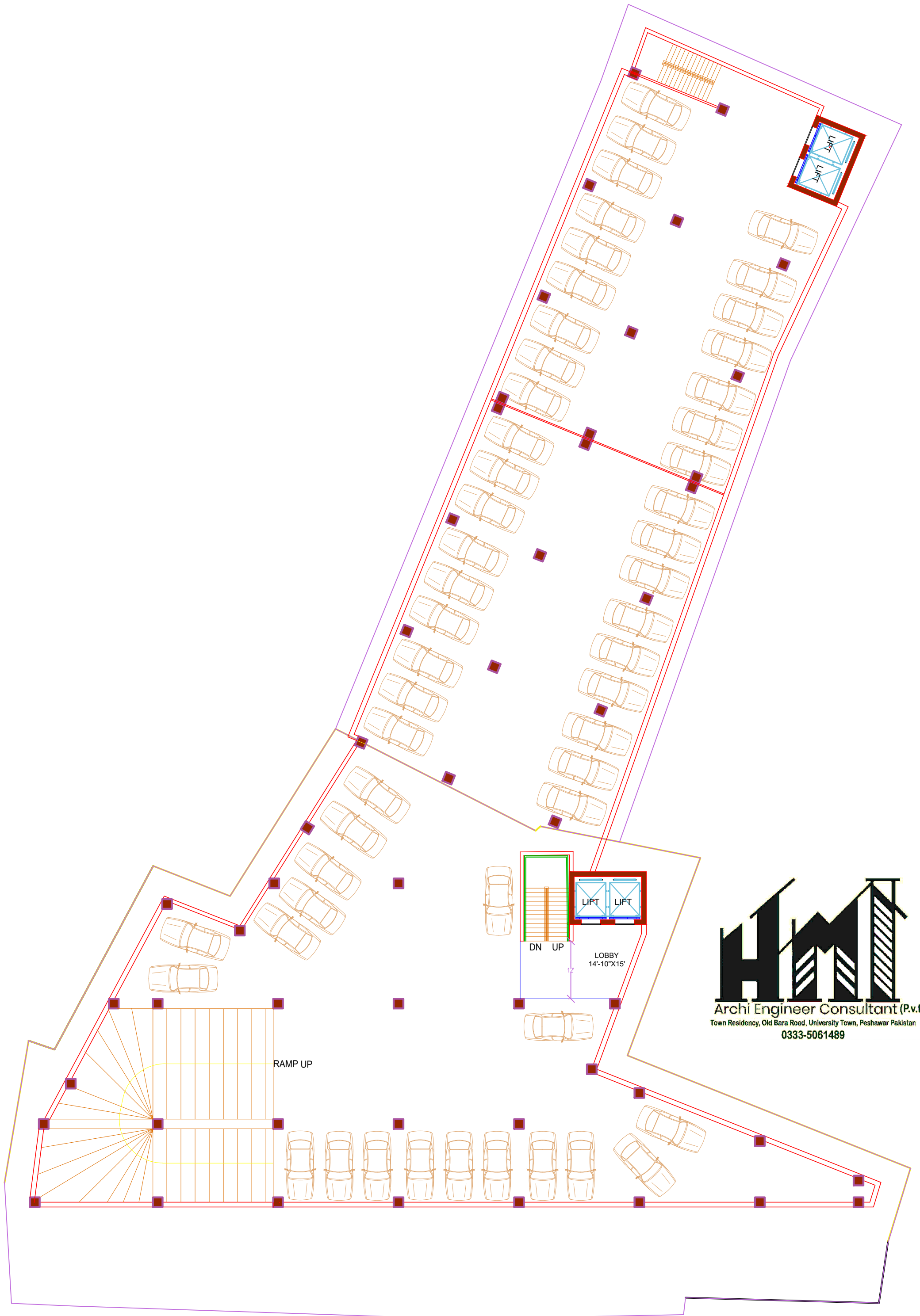
BASEMENT-3 PARKING
